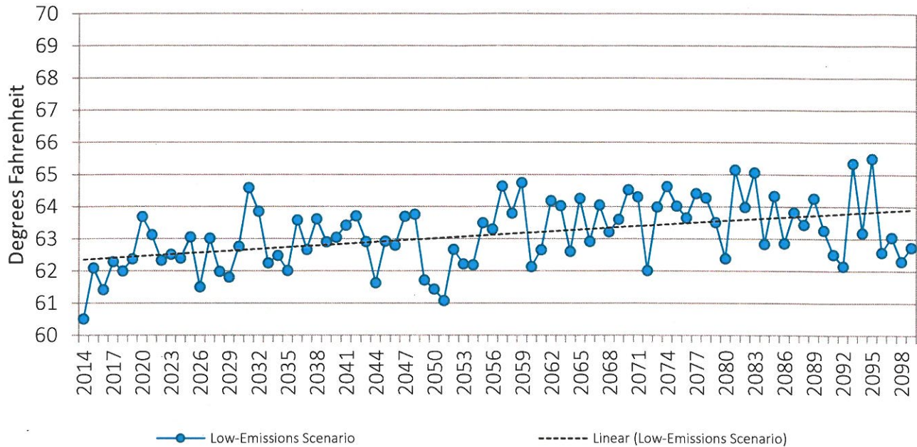
Figure 7: Projected Average Mean Temperatures, Low Emissions Scenario, 2014–2099
