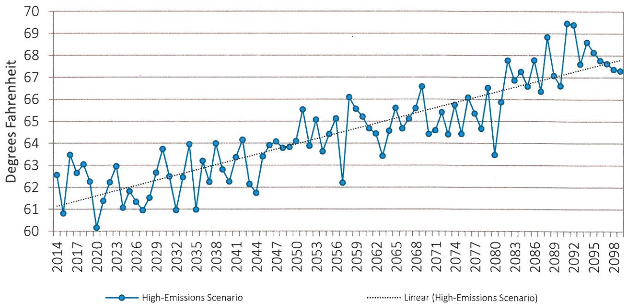
Figure 8: Projected Average Mean Temperatures, High Emissions Scenario, 2014–2099
