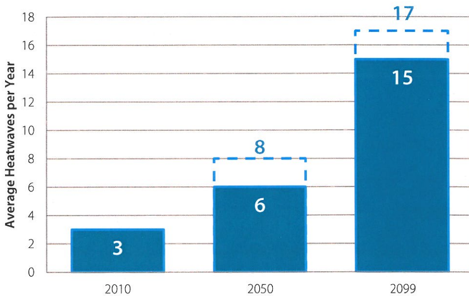
Figure 9: Projected Heat Waves per Year
